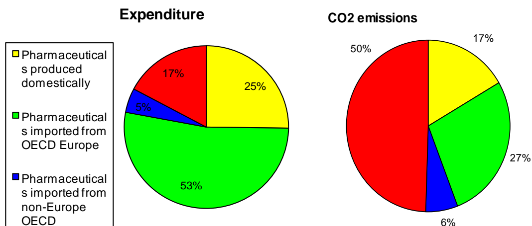
Figure 16: NHS spending on pharmaceutical products by origin and NHS embedded emissions from pharmaceutical products by origin 24 (raw data table in Appendix B2.11)
