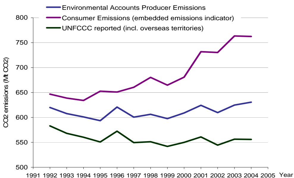
Figure 1: UK Carbon Dioxide Emissions (1992 to 2004) 18
