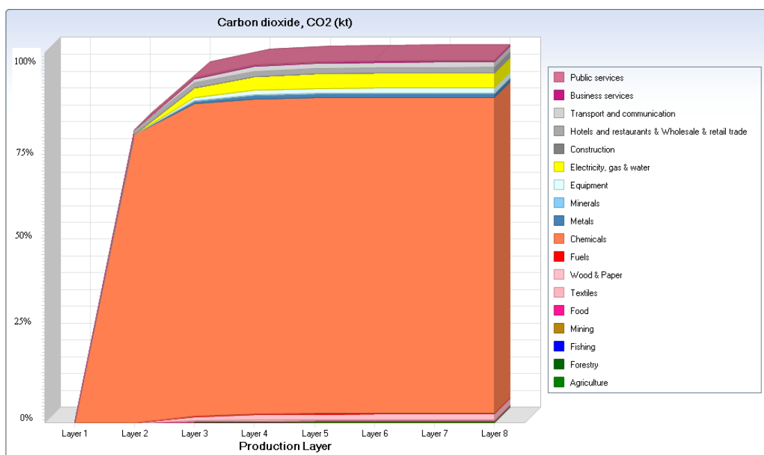
Figure 5: 2004 Pharmaceutical CO 2 emissions breakdown by production layer
