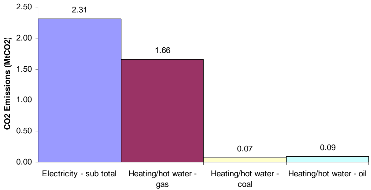
Figure 3 - 2004 CO 2 emissions: building energy sub-sectors
