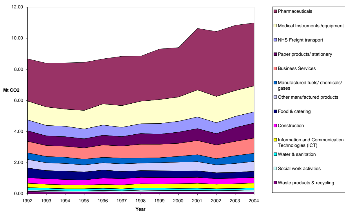
Figure 11 – Procurement sub-sector emissions 1992-2004
