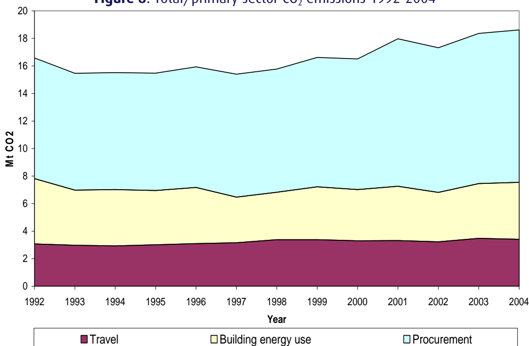
Figure 8: Total/primary sector CO 2 emissions 1992-2004
